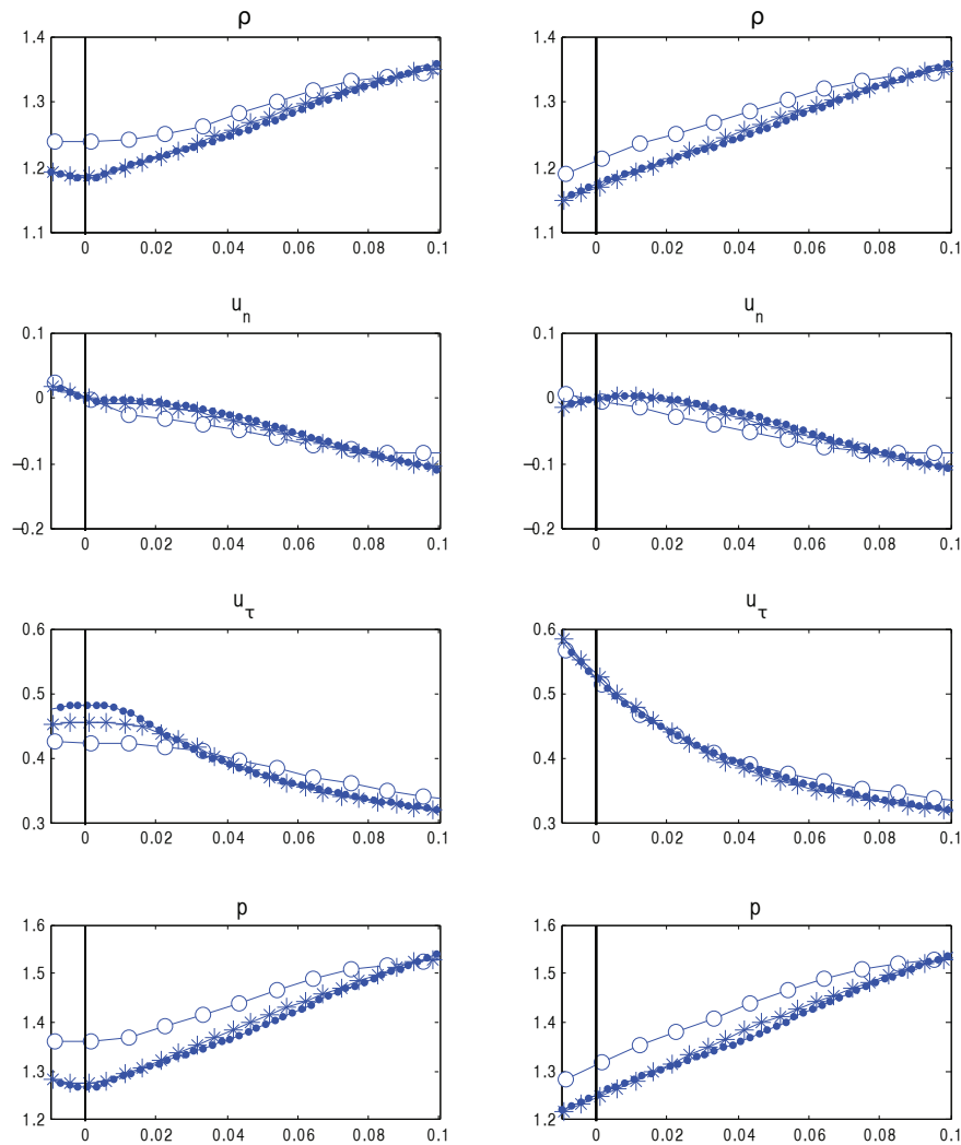
Figure 11: Example 2: Density, normal and tangential velocities and pressure as functions of the signed distance from the boundary in the vertical direction at t=0.2 . The results are computed by the proposed FD scheme with \Delta x = \Delta y = 1/50 (circles), 1/100 (stars) and 1/200 (dots) using the boundary conditions (3.8), (3.15), (3.11) and (3.12) (right) and the constant extrapolation (4.1) (left).
