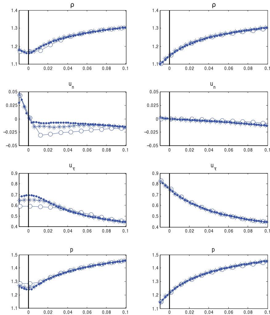
Figure 12: Example 3: Density, normal and tangential velocities and pressure as functions of the signed distance from the boundary in the vertical direction at t=0.4 . The results are computed by the proposed FD scheme with \Delta x=\Delta y=1/50 (circles), 1/100 (stars) and 1/200 (dots) using the boundary conditions (3.8), (3.15), (3.11) and (3.12) (right) and the constant extrapolation (4.1) (left).
