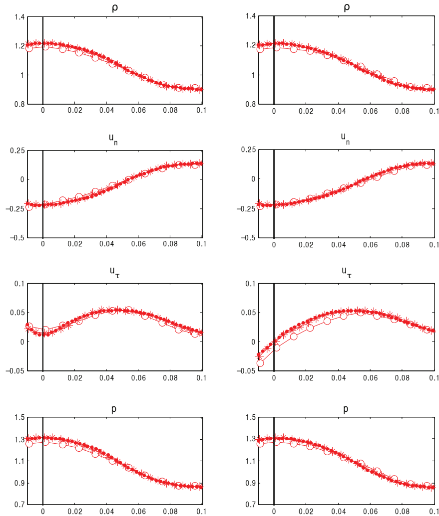
Figure 15: Example 4: Density, normal and tangential velocities and pressure as functions of the signed distance from the boundary in the oblique direction at t=0.2 . The results are computed by the proposed FD scheme with \Delta x = \Delta y = 1/50 (circles), 1/100 (stars) and 1/200 (dots) using the boundary conditions (3.21), (3.24), (3.23) and (3.12) (right) and the constant extrapolation (4.1) (left).
