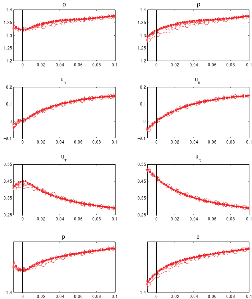
Figure 13: Example 3: Density, normal and tangential velocities and pressure as functions of the signed distance from the boundary in the oblique direction at t=0.4 . The results are computed by the proposed FD scheme with \Delta x = \Delta y = 1/50 (circles), 1/100 (stars) and 1/200 (dots) using the boundary conditions (3.8), (3.15), (3.11) and (3.12) (right) and the constant extrapolation (4.1) (left).
