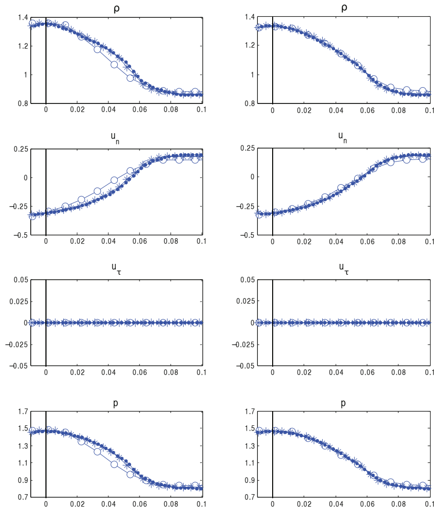
Figure 14: Example 4: Density, normal and tangential velocities and pressure as functions of the signed distance from the boundary in the vertical direction at t=0.2 . The results are computed by the proposed FD scheme with \Delta x = \Delta y = 1/50 (circles), 1/100 (stars) and 1/200 (dots) using the boundary conditions (3.21), (3.24), (3.23) and (3.12) (right) and the constant extrapolation (4.1) (left).
