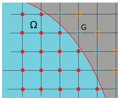
Figure 3: Grid points setup: The red filled circular points are inner points, the light blue unfilled circular and yellow unfilled square points are the first and second layers of ghost points, respectively.
