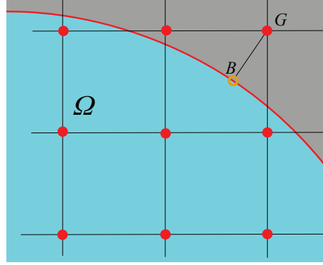
Figure 5: Ghost point G \in \mathcal{L}_1 , its boundary projection B \in \partial\Omega , and the stencil \mathcal{S}_G (red filled circular points).
