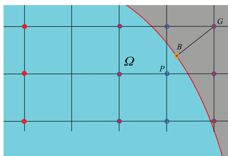
Figure 6: Enlarged stencil \mathcal{S}_G for the ghost point G : since \alpha_x = \frac{|x_B - x_P|}{\Delta x} is below a prefixed threshold, the original stencil (blue unfilled circular points) is enlarged in the x -direction (red filled circular points).
