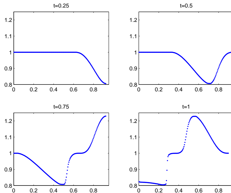
Figure 8: Example 1: Density computed using the proposed FD scheme at four different times.
