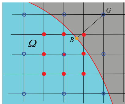
Figure 7: Ghost point G \in \mathcal{L}_2 , its boundary projection B \in \partial\Omega , and two stencils: S_G^I (red filled circular points) and S_G^{II} (blue unfilled circular points).
