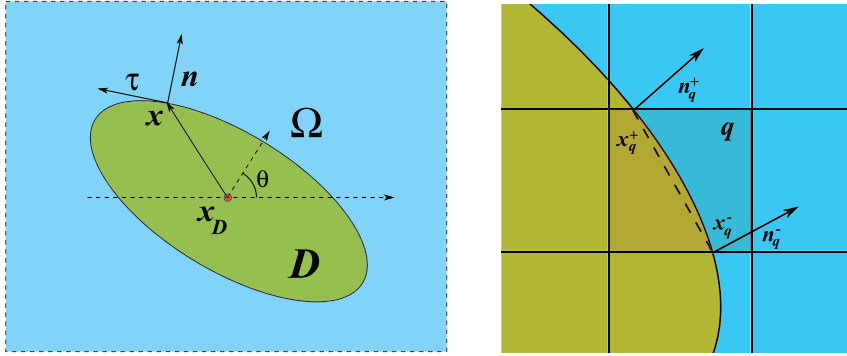
Figure 17: Setting for the computation of the total force and torque, obtained by integrating along the boundary of the object D (left); the square q , segment \Delta\Gamma_q (dashed line) and unit normals at the end points used for the computation of a contribution to the total force F and torque T (right).
