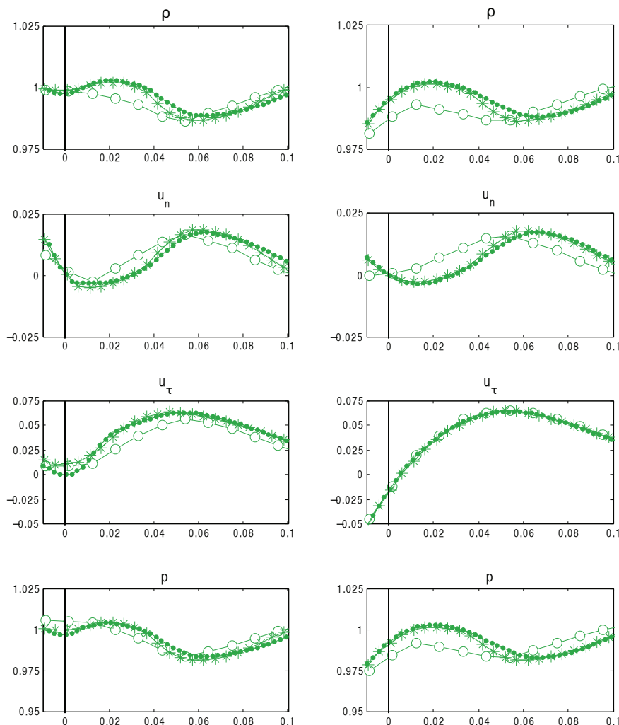
Figure 16: Example 4: Density, normal and tangential velocities and pressure as functions of the signed distance from the boundary in the oblique direction at t=0.2 . The results are computed by the proposed FD scheme with \Delta x = \Delta y = 1/50 (circles), 1/100 (stars) and 1/200 (dots) using the boundary conditions (3.21), (3.24), (3.23) and (3.12) (right) and the constant extrapolation (4.1) (left).
