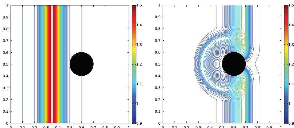
Figure 10: Example 2: Density computed by the proposed FD scheme at times t=0 (left) and t=0.2 (right).
