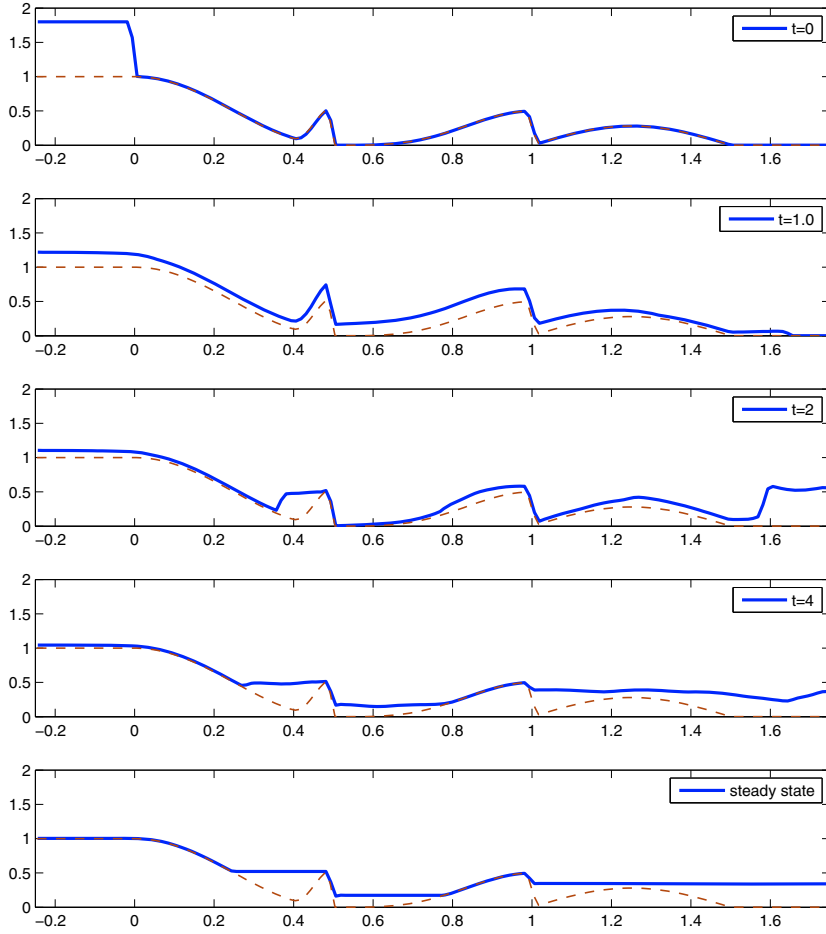
FIGURE 14. 1-D slice of the water level w (solid line) and the interpolated bottom B (dashed line) from the 2 \times 200 \times 200 numerical solution shown in Figure 13.
